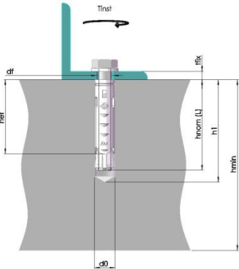
Figure A3: Installed FM-MP3®evo anchor
