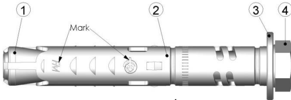
Figure A1: FM-MP3®evo anchor
