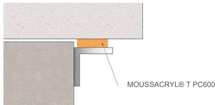
Croquis 2 : Joint solin
